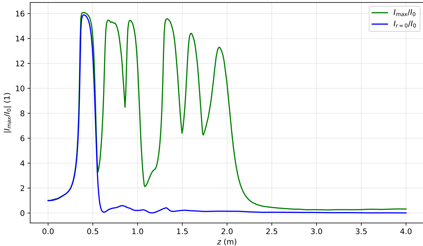
I_{max}(x=0, y=0, z)/I_0 , Pin=6.9Pcr, noisy input, artificial time
